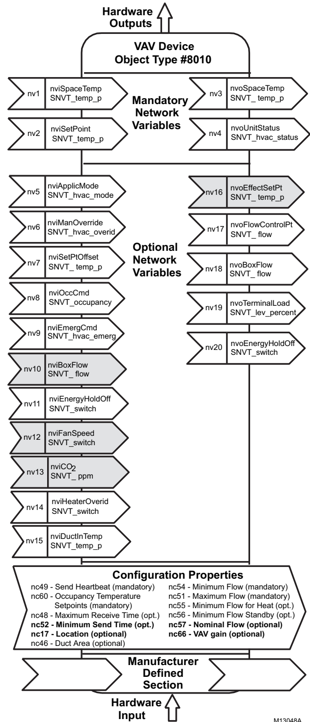
Fig. 1. Functional profile of LonMark VAV object details (variables not implemented in Excel 10 VAV Controllers are grayed, or in bold print in Configuration Properties).
